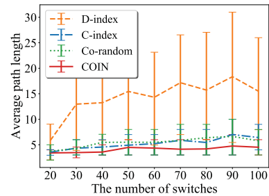
Fig. 9. The impact of multiple index copies on the average path lengths.
